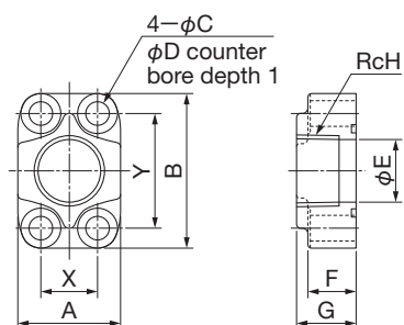
Screw joint pipe flange
