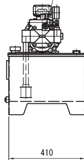
Dimension table (Unit: mm)
